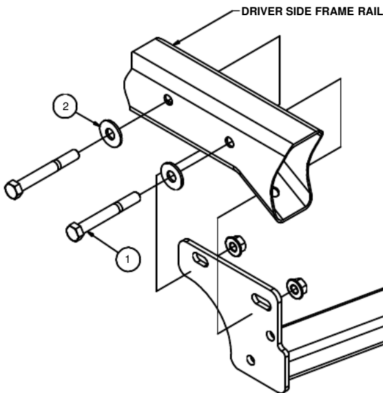
INSTALLED POSITION
